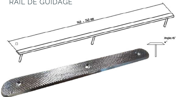
RAIL DE GUIDAGE
